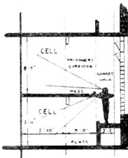
TYPICAL SECTION THRU CELLS
