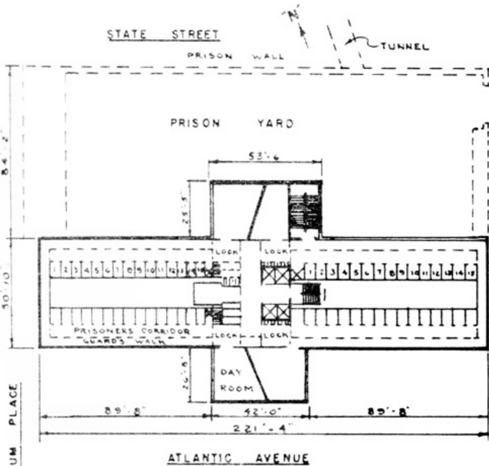
TYPICAL PLAN ( 4, 5, 6, 7, 8 & 9 th FL.)
